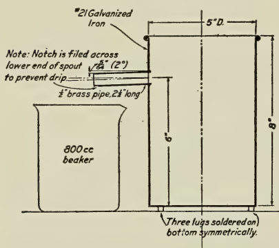
FIG. 192.—Goldbeck's Specific Gravity Apparatus.
